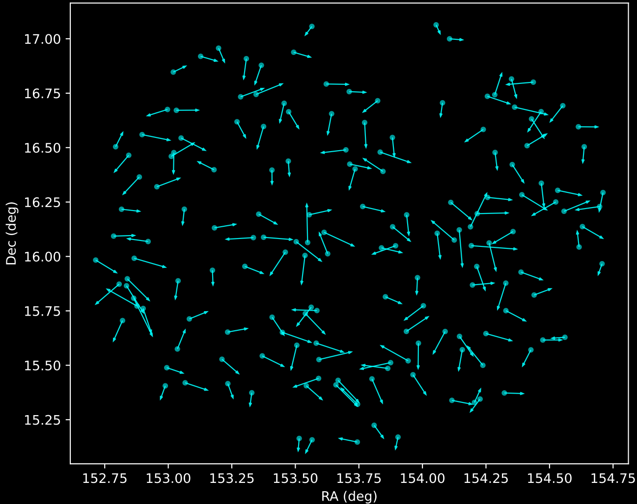
GALAH DR4 Noise Stream Proper Motion Vectors (n=162)
