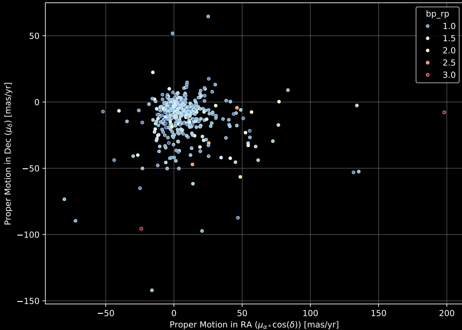
GALAH DR4 Field: [6601] Proper Motion Diagram (n= 462)
