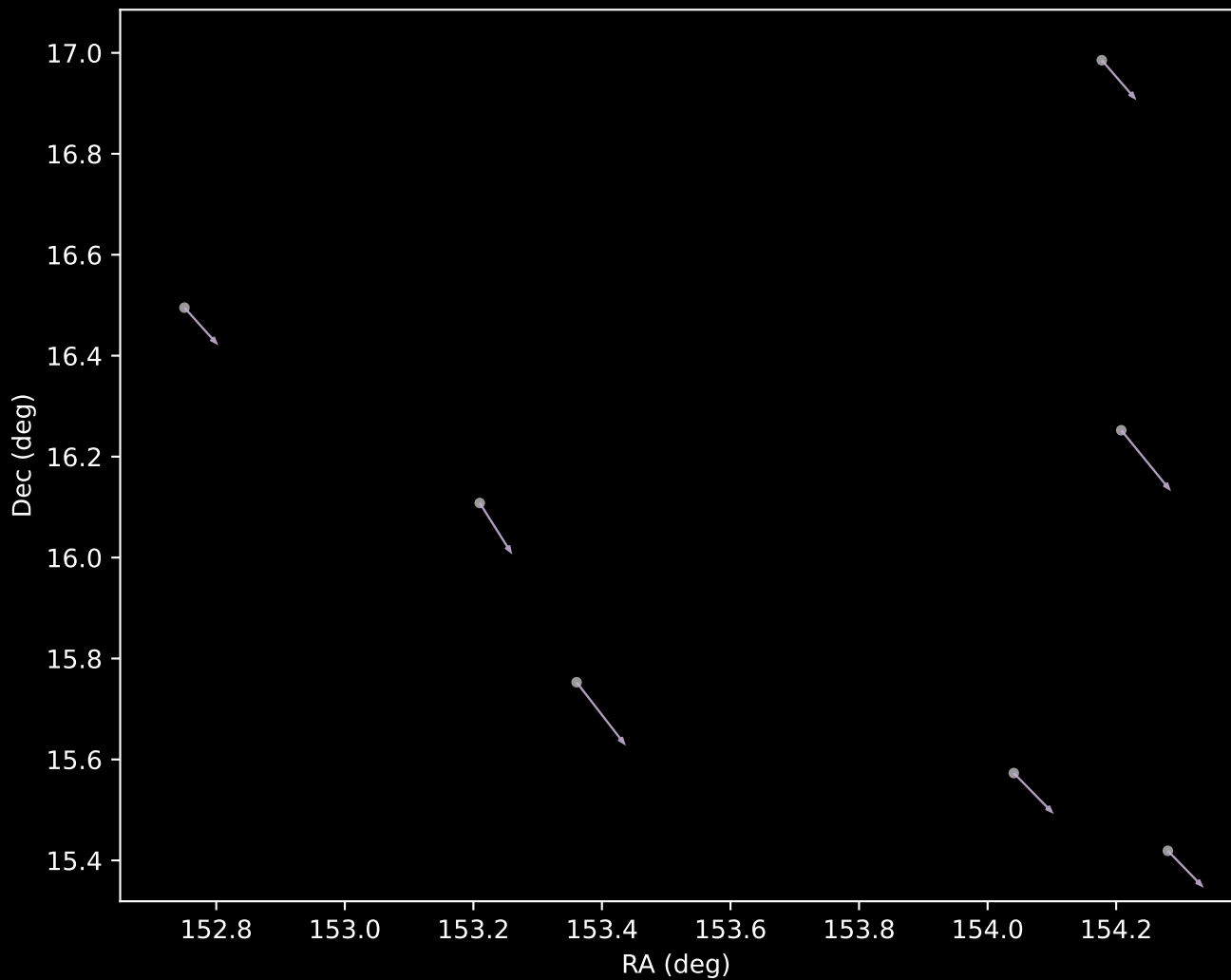
GALAH DR4 Cluster 9 Proper Motion Vectors (n=7)
