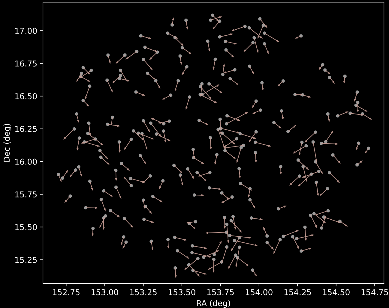
GALAH DR4 Cluster 11 Proper Motion Vectors (n=223)
