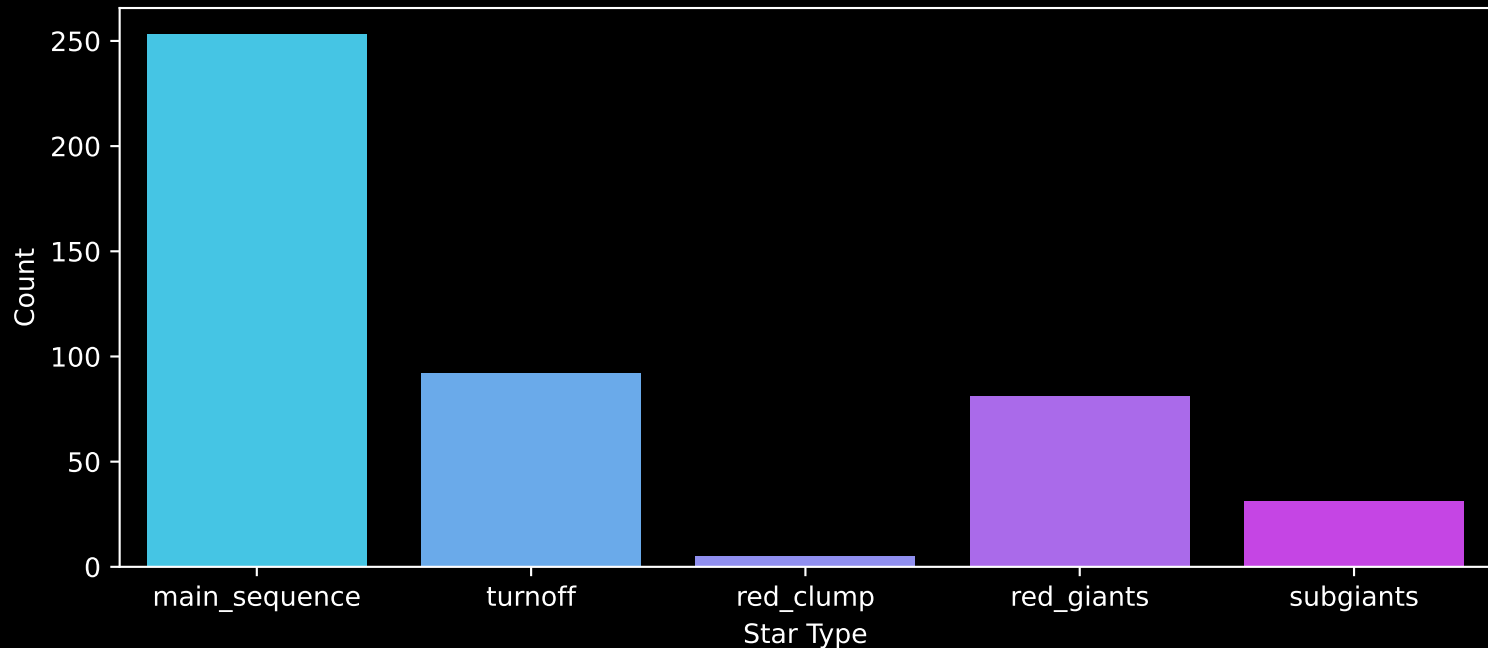
GALAH DR4 Field: [6601] Count plot of Star Type
