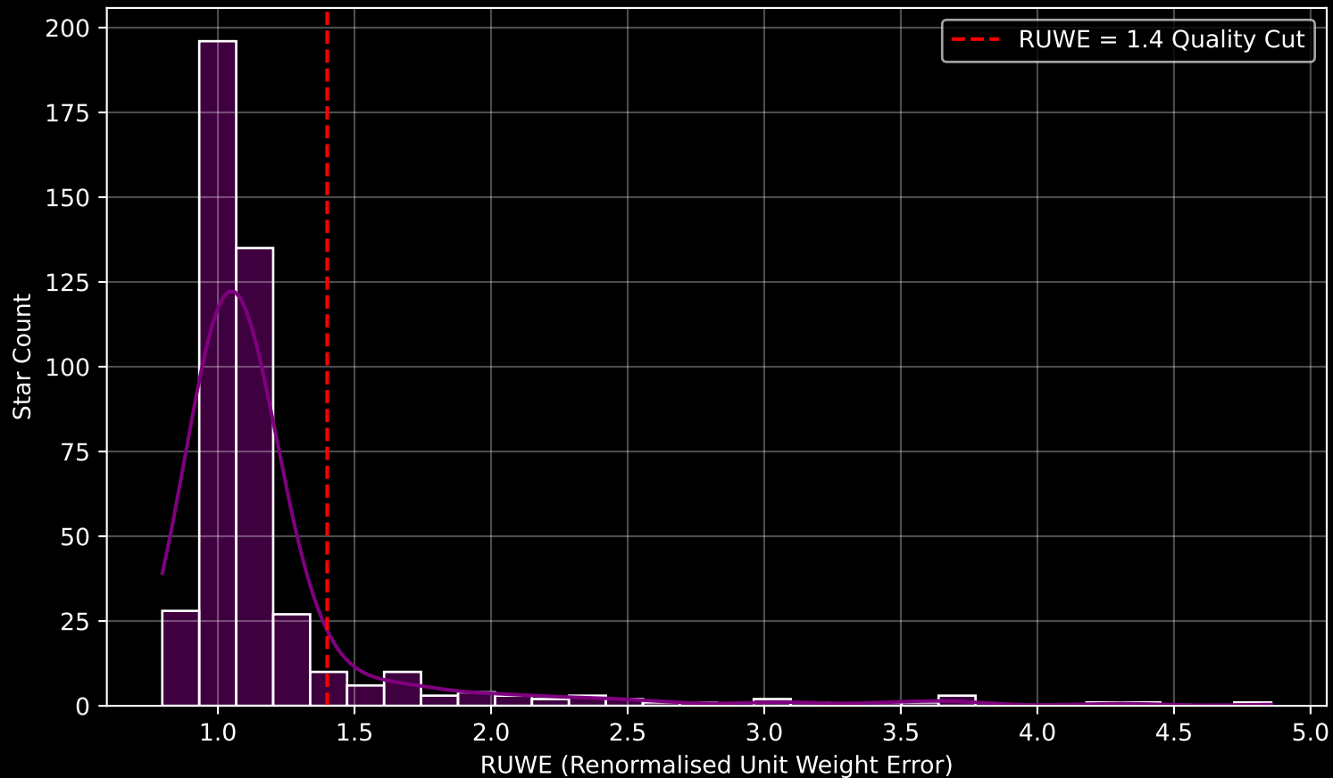
GALAH DR4 Field [6601] RUWE Distribution (n= 442)
